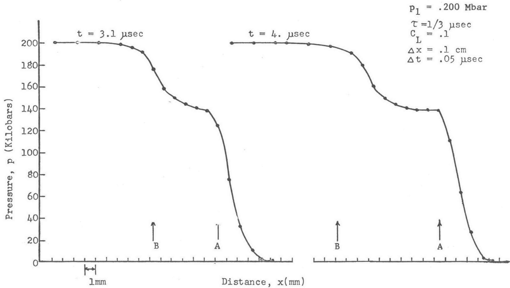
Fig. 5.5. --Double-Shock in Iron. \Delta x and \Delta t are space and time increments used in the numerical integration.
